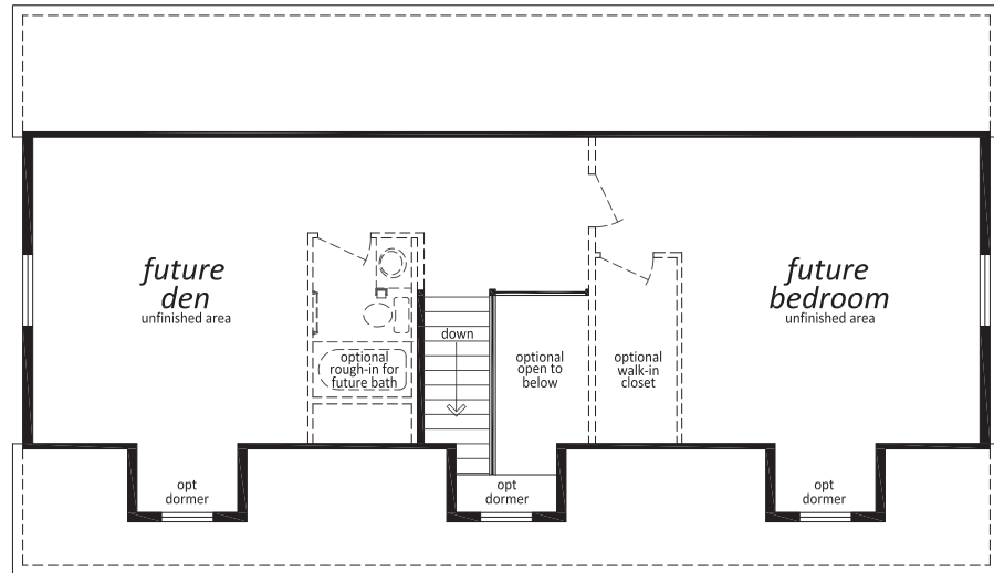
Second Floor 736 sq. ft. (Approx.)
