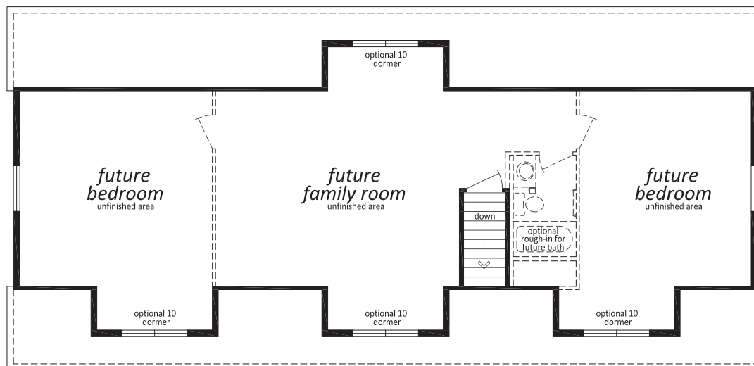
Second Floor 889 sq. ft. (Approx.)
